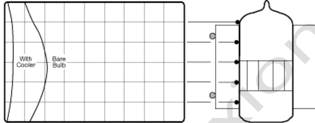
MCF-7: 7-pin Miniature Cooling Performance
