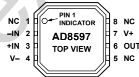
Figure 1. AD8597 8-Lead SOIC (R-8)
