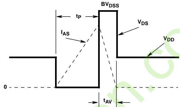
FIGURE 16. UNCLAMPED ENERGY WAVEFORMS
